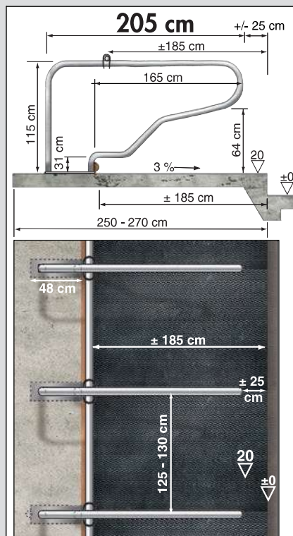
Dimensions for cubicle Classic installation as high bed cubicle for heavy livestock
