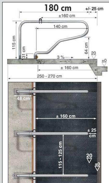
Dimensions for cubicle Classic installation as high bed cubicle for heifers
