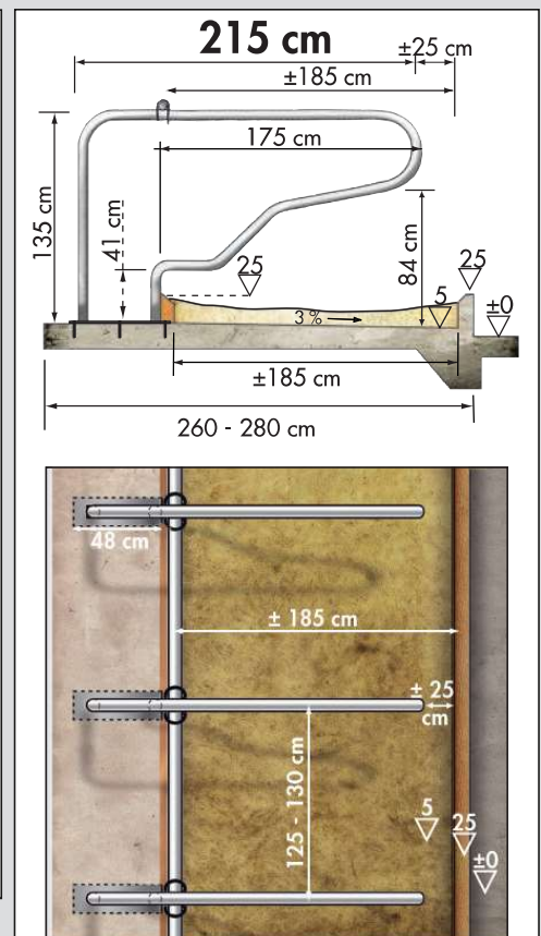
Dimensions for cubicle Classic installation as deep bed cubicle for heavy livestock
