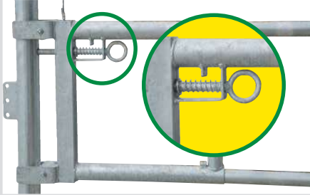
Even more stability due to welded tubes Locking trough spring-loaded bolts
