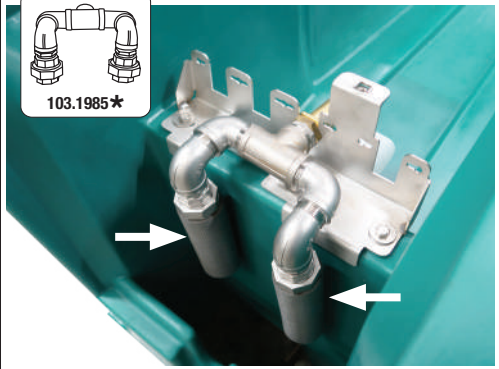
Connection possiblitiy to water circuit
